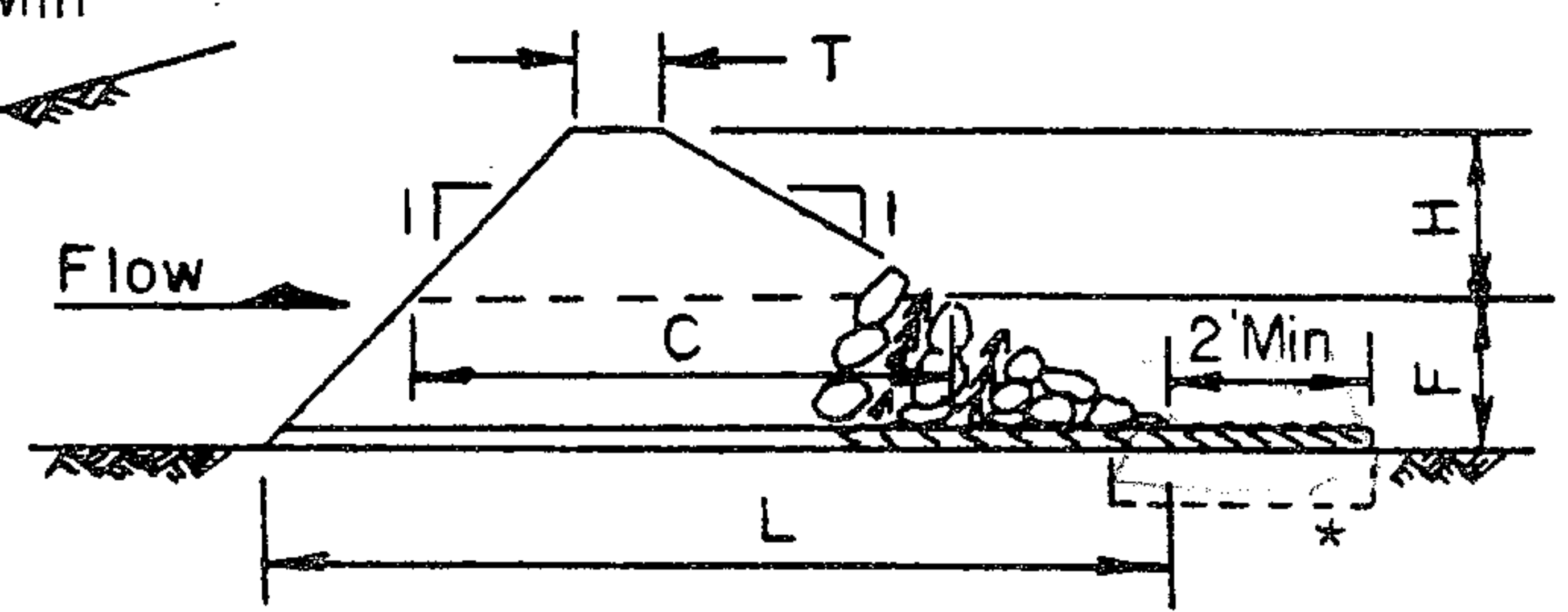
SECTION B-B
