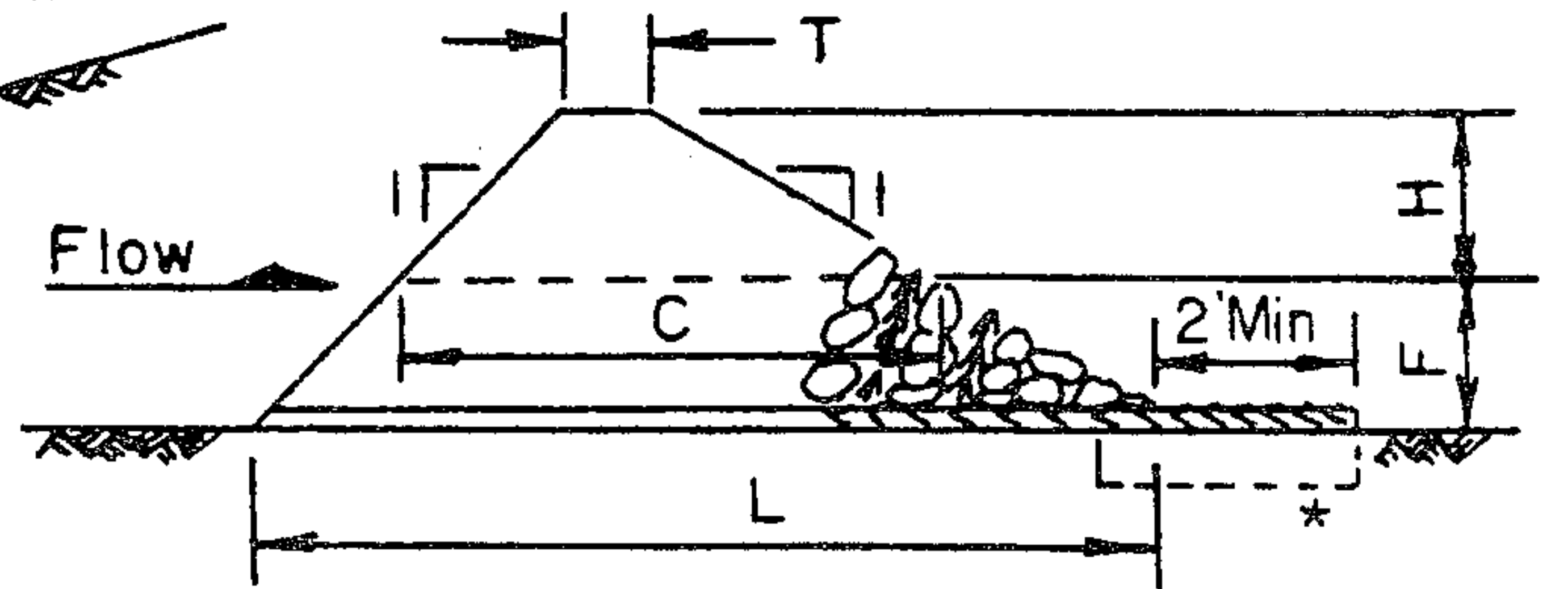
SECTION B-B
