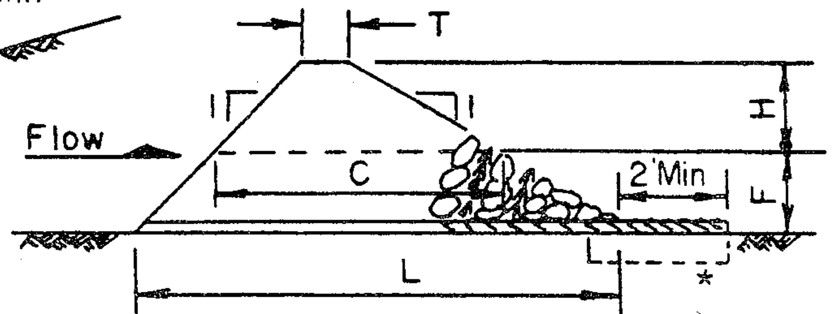
SECTION B-B
