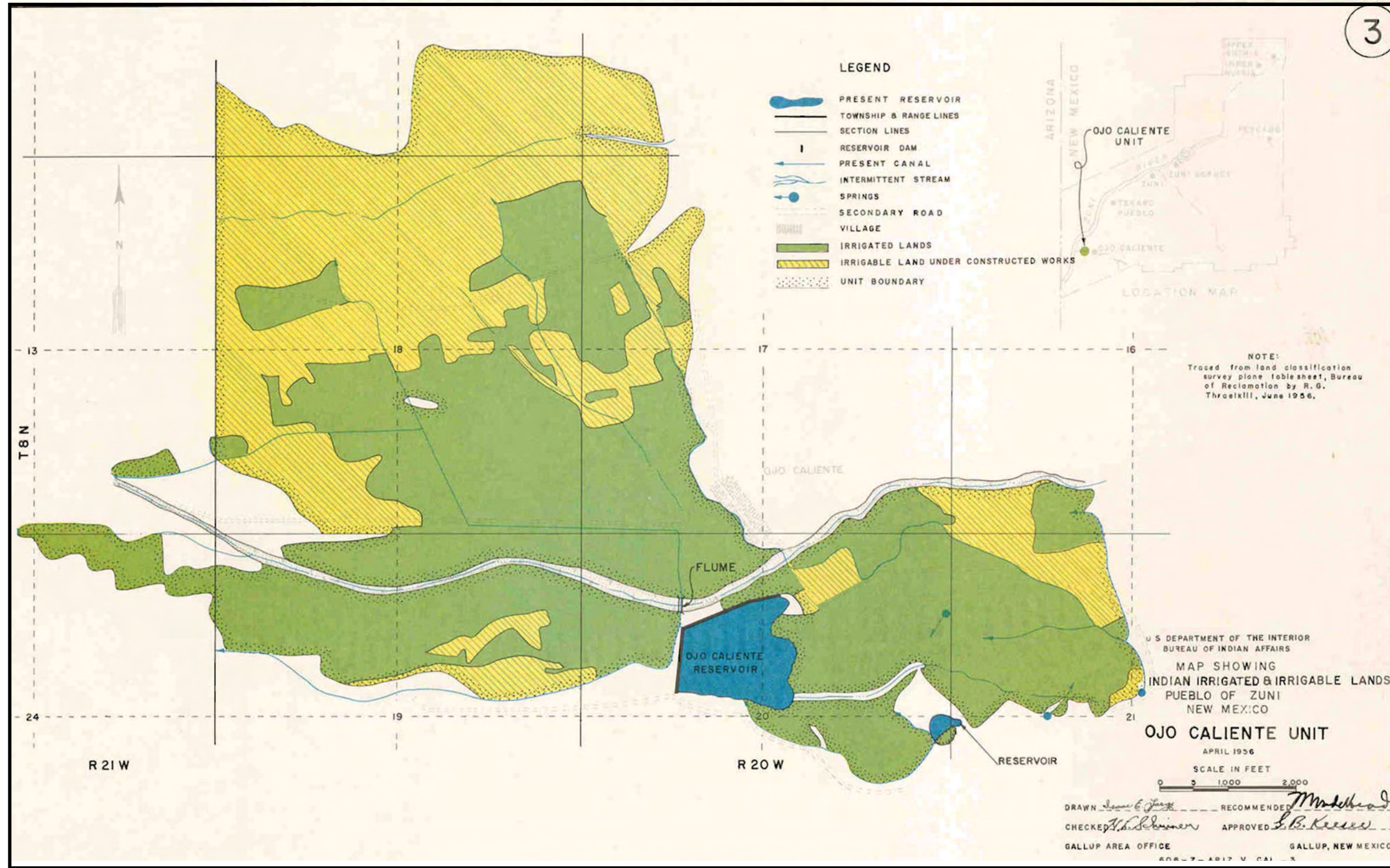
Figure B-3: Ojo Caliente Unit, Irrigated and Irrigable Lands Map
