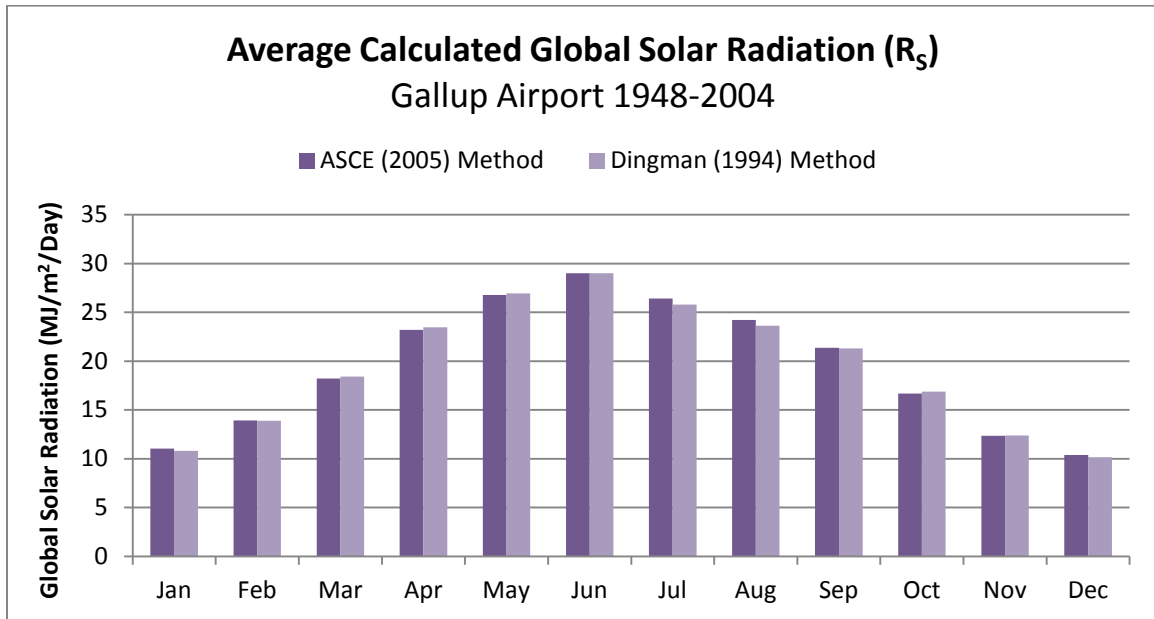
Figure 18 – Comparison of Global Solar Radiation at Gallup Airport (1948-2004) Calculated with Dingman (1994) and ASCE (2005) Equations, filled from Albuquerque Int’l as described in section 2.5.1
