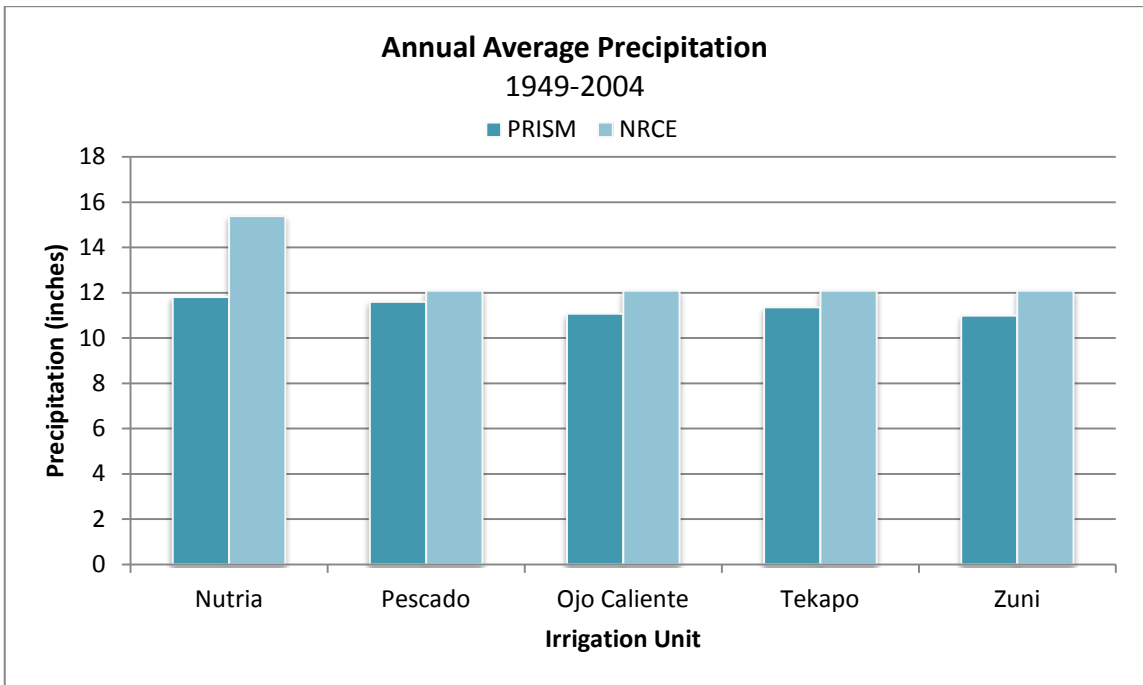
Figure 12 - PRISM vs. NRCE Analysis for Average Annual Precipitation
