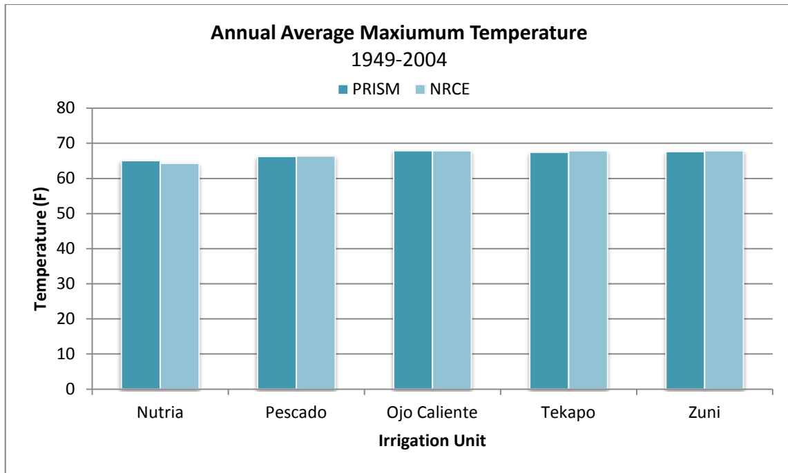
Figure 9 - PRISM vs. NRCE Analysis for Maximum Temperature
