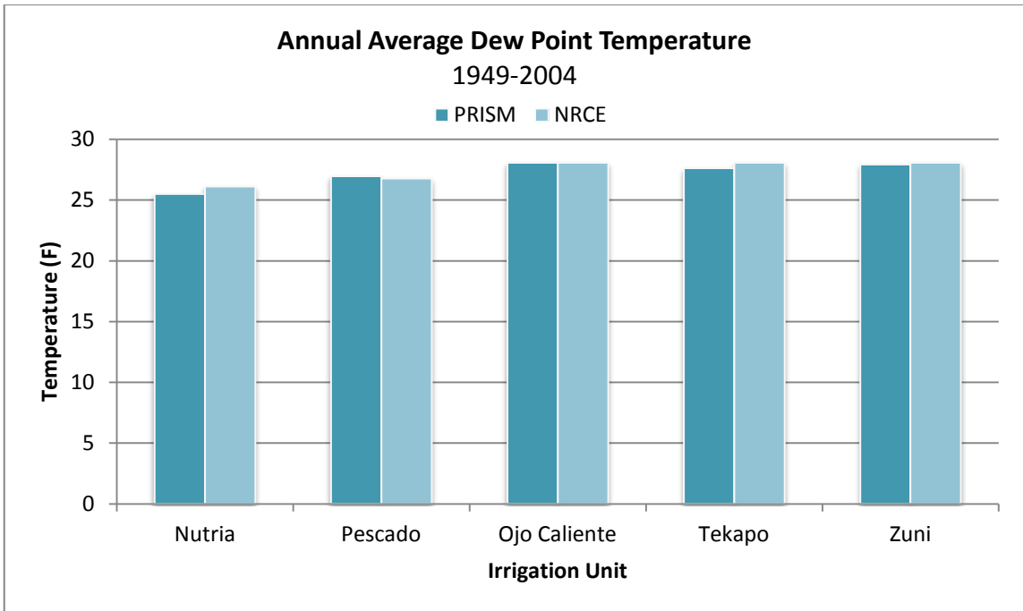
Figure 11 - PRISM vs. NRCE Analysis for Dew Point Temperature
