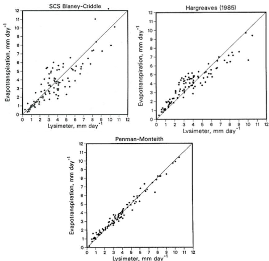
Figure 15 - Estimated ET versus Measured ET (lysimeter) for Blaney-Cridde, Hargreaves, and Penman-Monteith Methods at 11 Locations (Jensen, et al., 1990)
