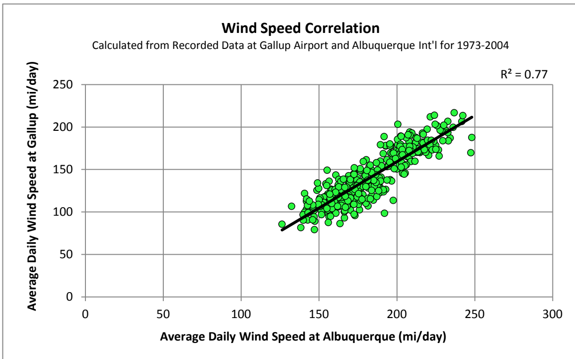
Figure 4 - Average Daily Wind Speed Correlation between Gallup and Albuquerque
