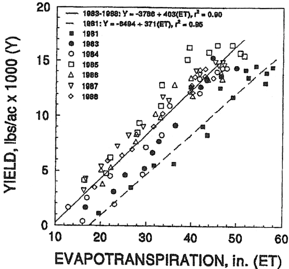
Figure 16 - Crop production function for alfalfa (Smeal, 1995)
