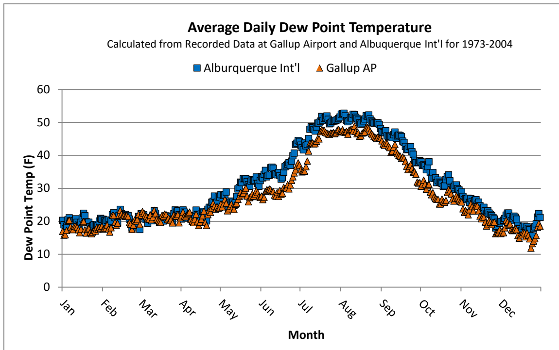
Figure 1 – Average Daily Dew Point Temperature ( T_{dew} ) at Gallup and Albuquerque
