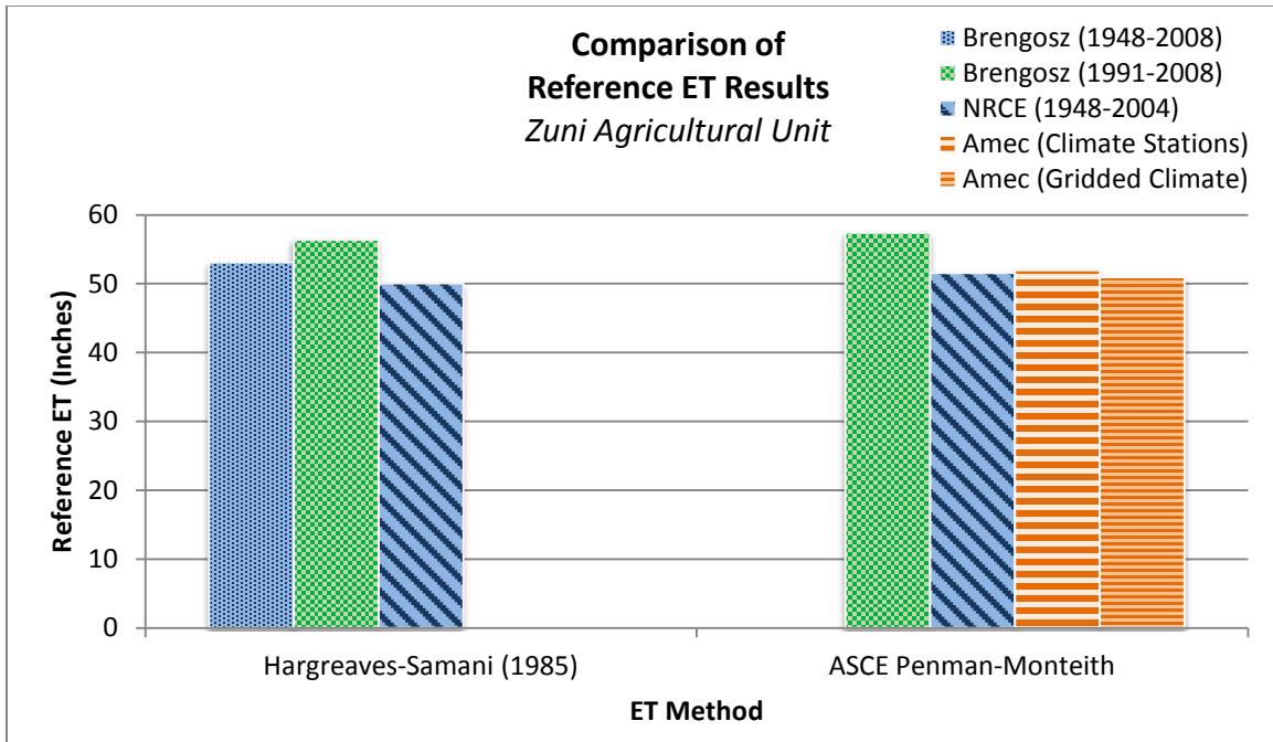
Figure 14 - Comparison of Experts' Reference ET Estimates for Zuni
