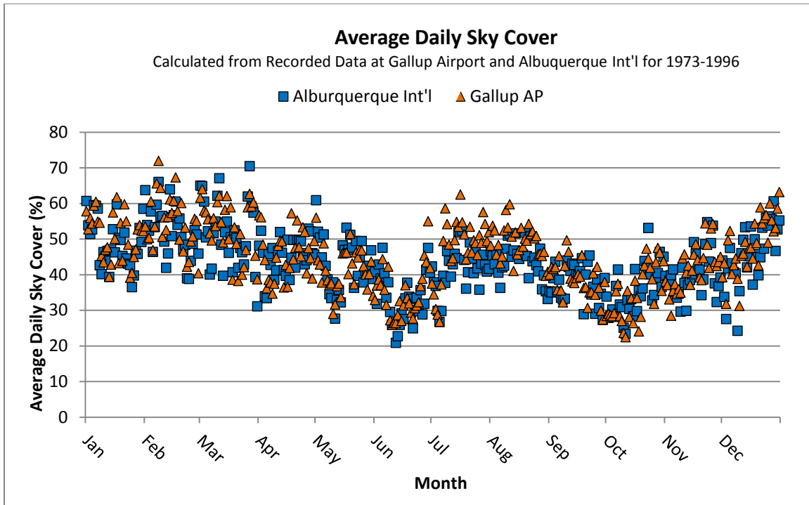
Figure 5 - Average Daily Sky Cover at Gallup and Albuquerque 1973-1996
