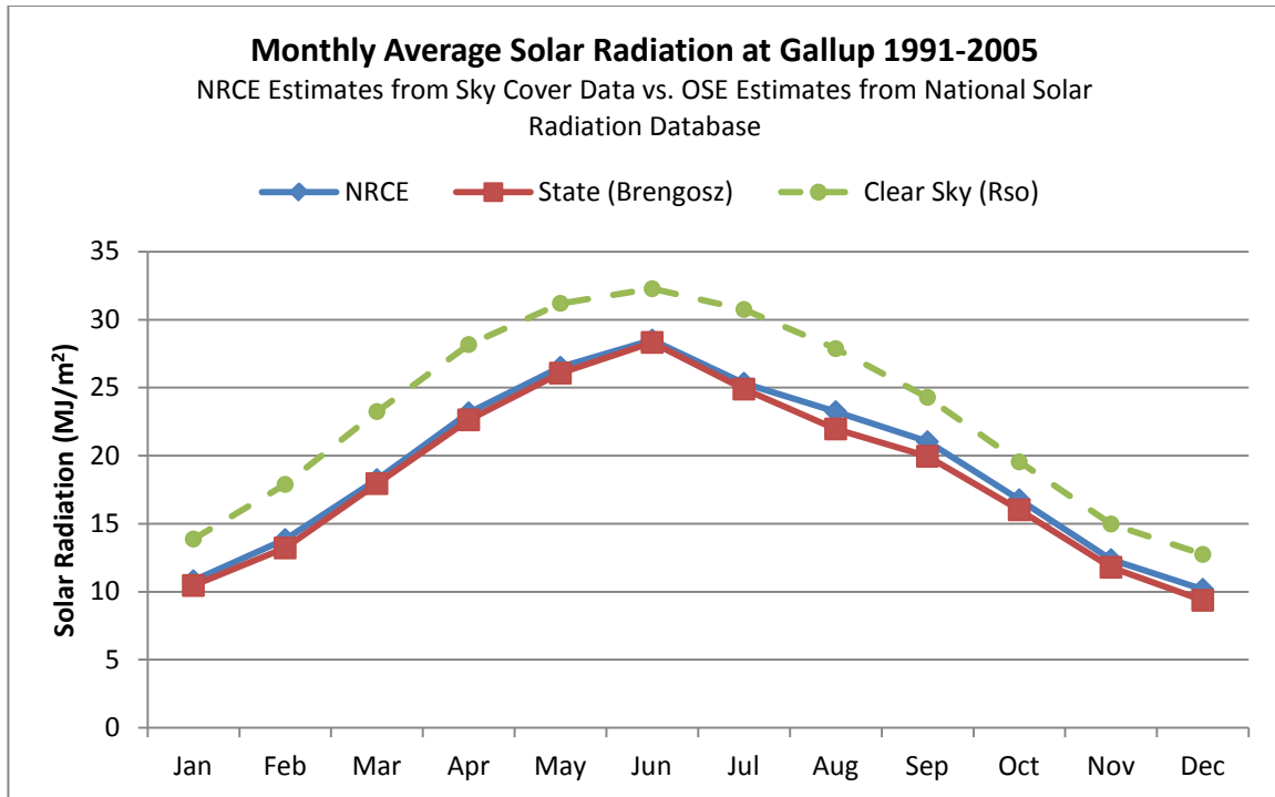
Figure 8 - Monthly Solar Radiation at Gallup, Estimates from NRCE's Sky Cover Data vs. Bregosz (2010)'s Radiation Estimates from NSRDB
