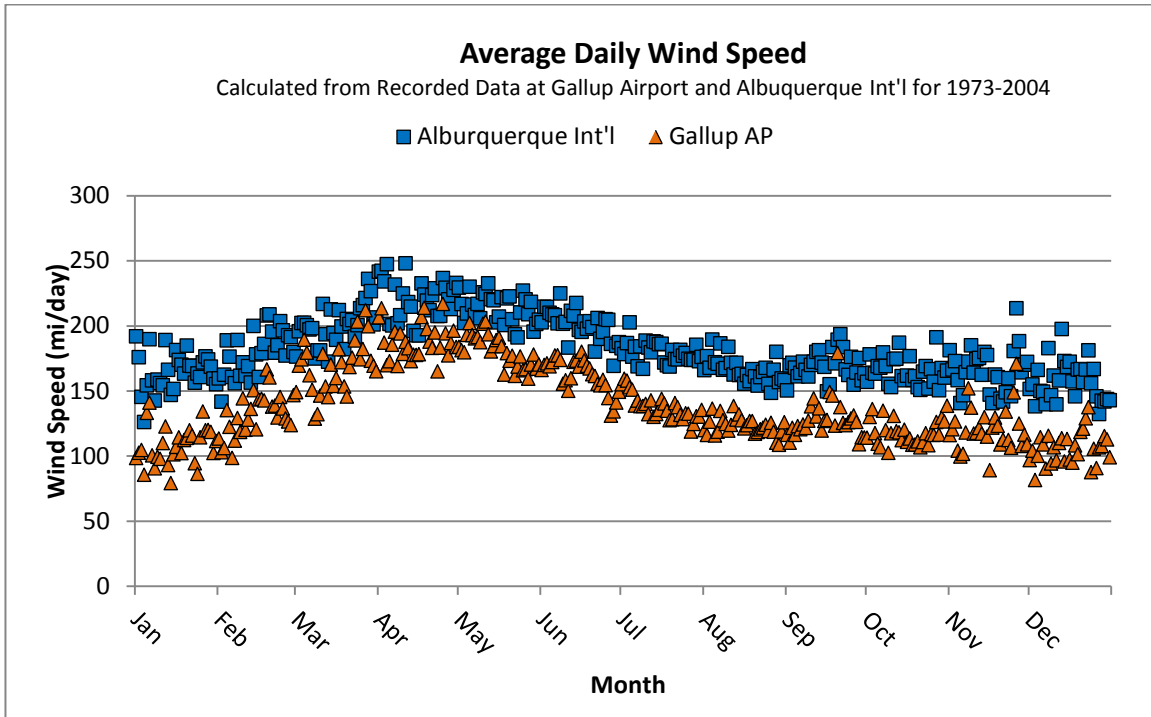
Figure 3 - Average Daily Wind Speed at Gallup and Albuquerque
