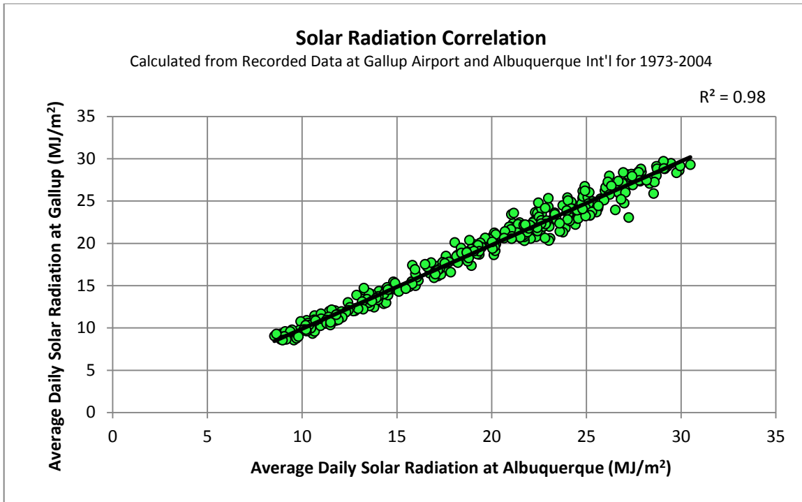
Figure 7 - Average Daily Solar Radiation Correlation between Gallup and Albuquerque
