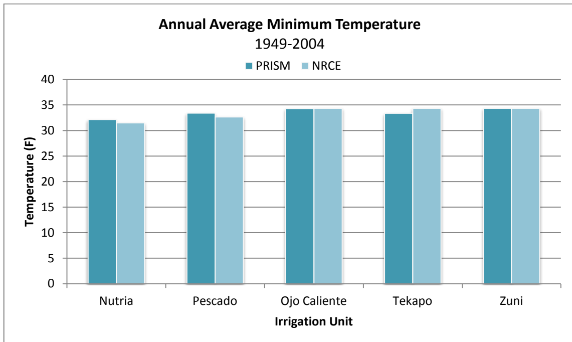
Figure 10 - PRISM vs. NRCE Analysis for Minimum Temperature
