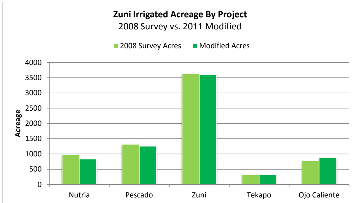
Figure 23 - 2008 NRCE Survey Acreage vs. 2011 Modified Acreage
