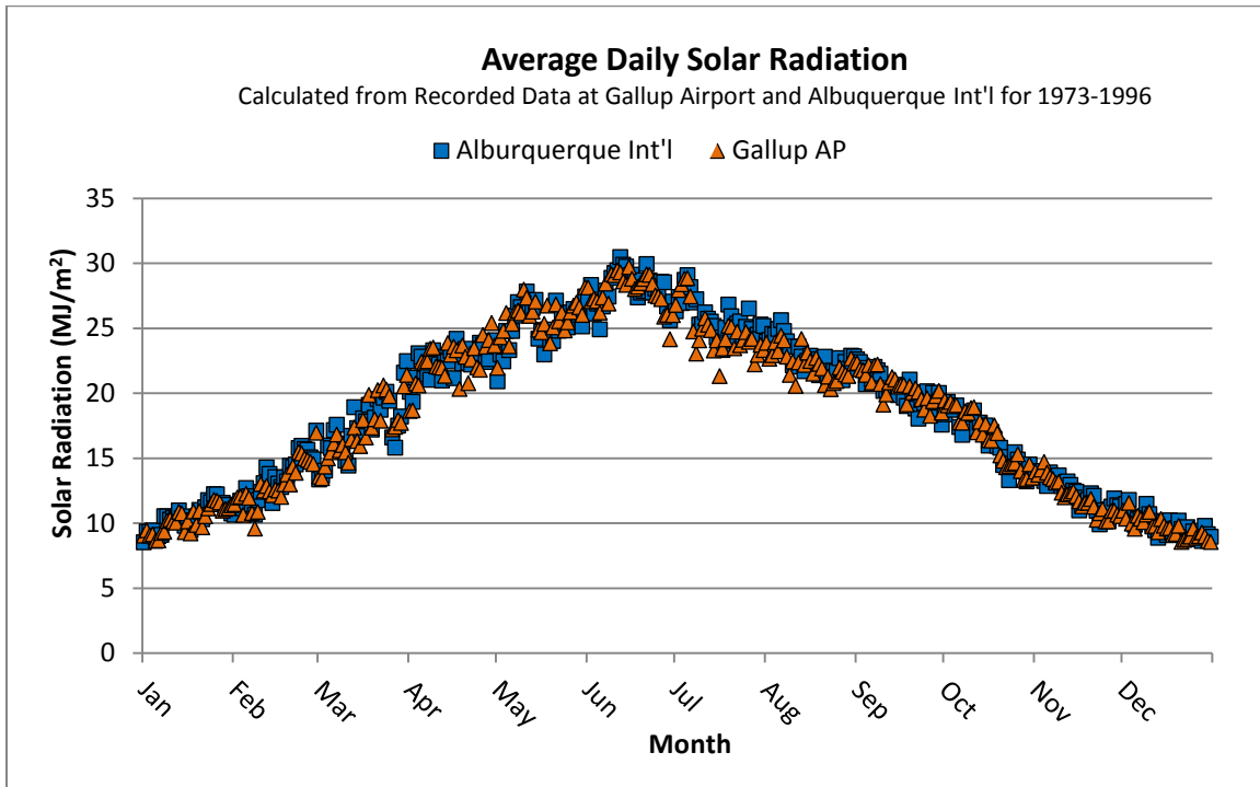
Figure 6 - Average Daily Solar Radiation at Gallup and Albuquerque 1973-1996
