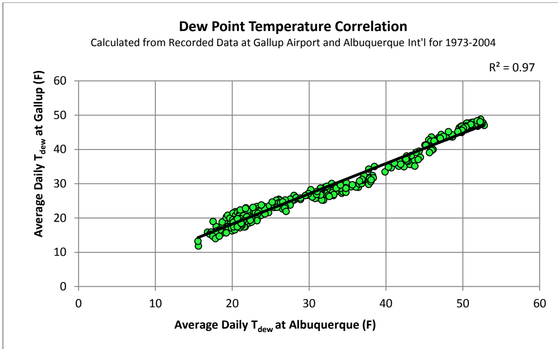
Figure 2 - Average Daily Dew Point Temperature ( T_{dew} ) Correlation between Gallup and Albuquerque
